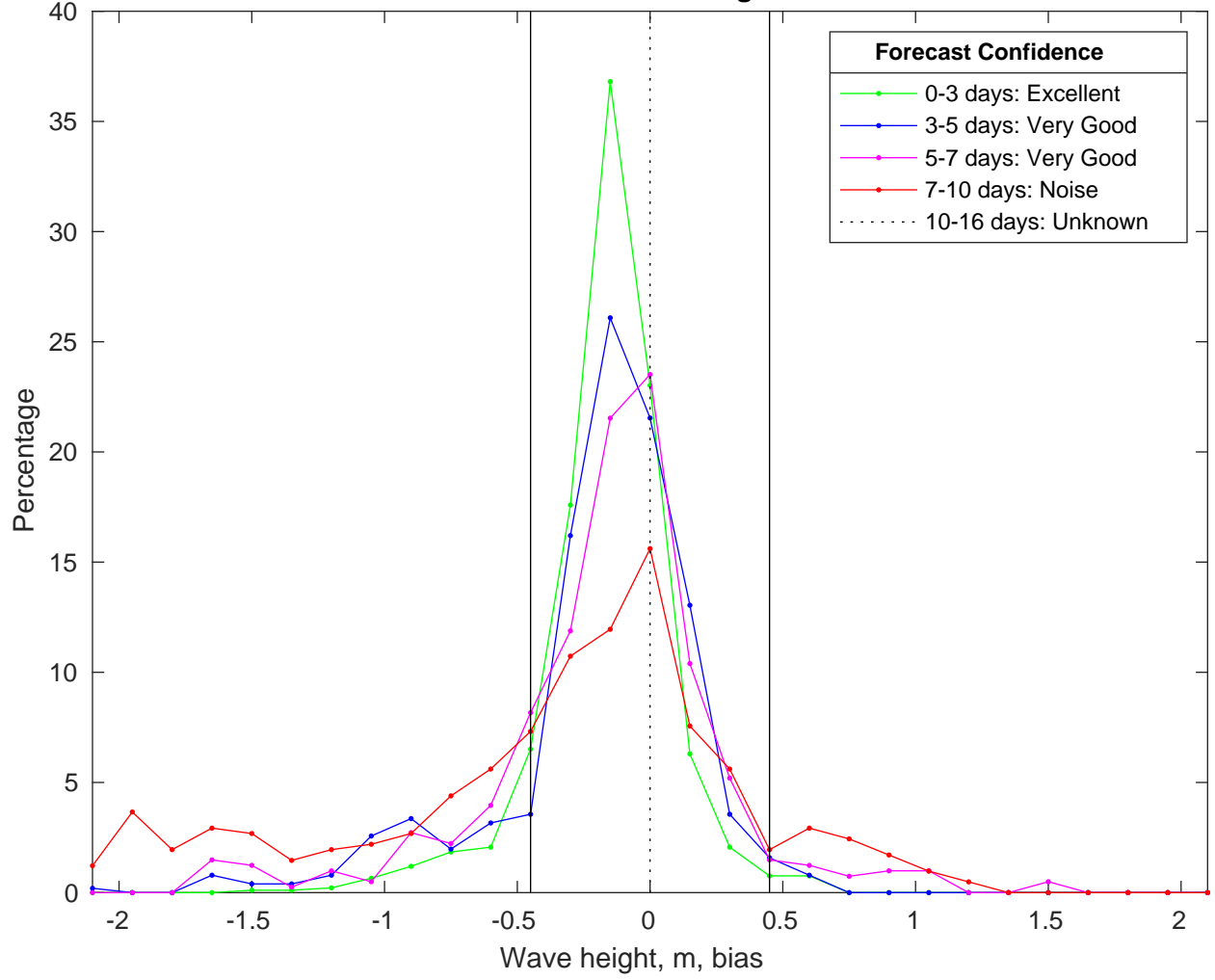
NDBC 42040 vs CMEMSWaves Bias Histogram: 12-Jan-2025
