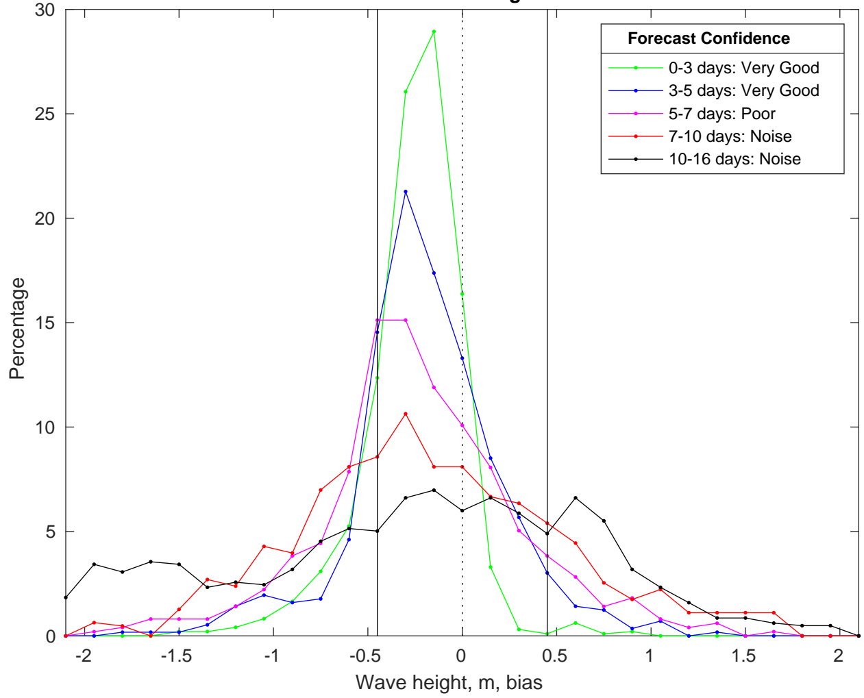
NDBC 42040 vs GFSWaves Bias Histogram: 12-Jan-2025
