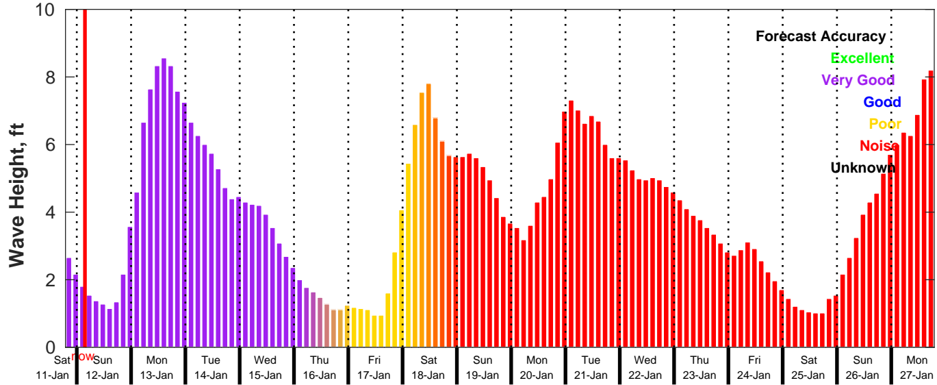
GFS Wave Forecast for NDBC 42040 from 11-Jan-2025 19:00:00 to 27-Jan-2025 19:00:00
