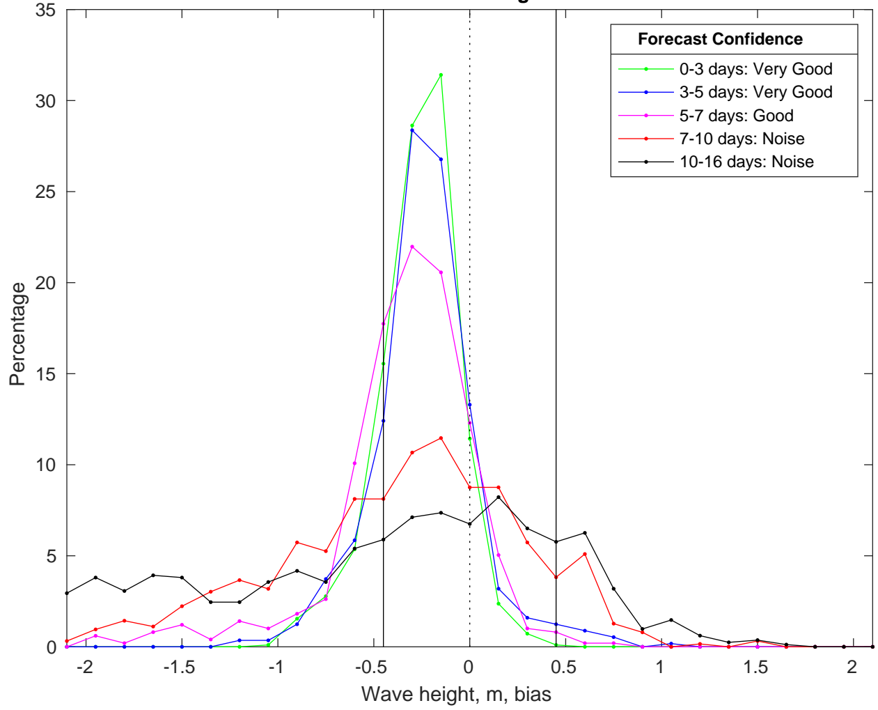
NDBC 42084 vs GFSWaves Bias Histogram: 12-Jan-2025
