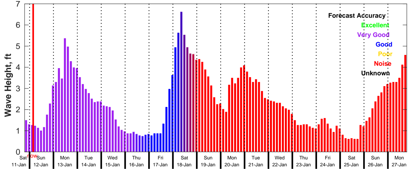
GFS Wave Forecast for NDBC 42084 from 11-Jan-2025 19:00:00 to 27-Jan-2025 19:00:00
