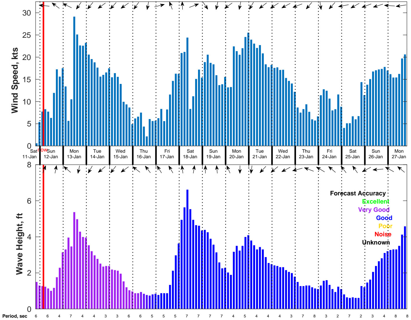
Wind & Wave Forecast for NDBC 42084 from 11-Jan-2025 19:00:00 to 27-Jan-2025 19:00:00
