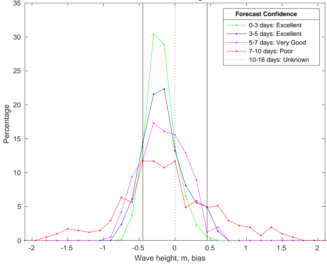
NDBC 42092 vs CMEMSWaves Bias Histogram: 12-Jan-2025
