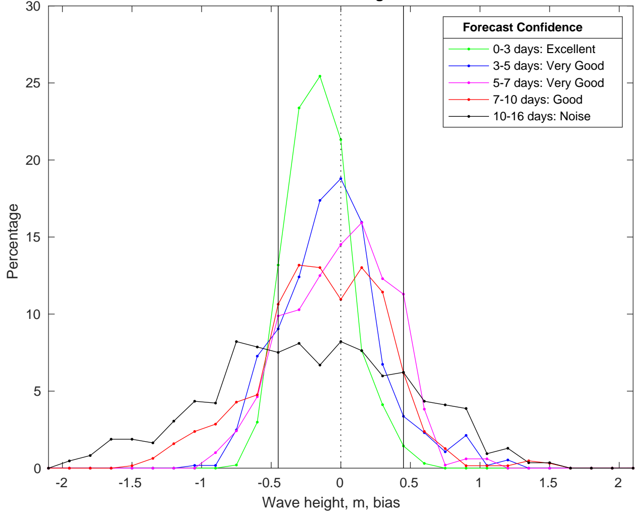
NDBC 42092 vs GFSWaves Bias Histogram: 12-Jan-2025
