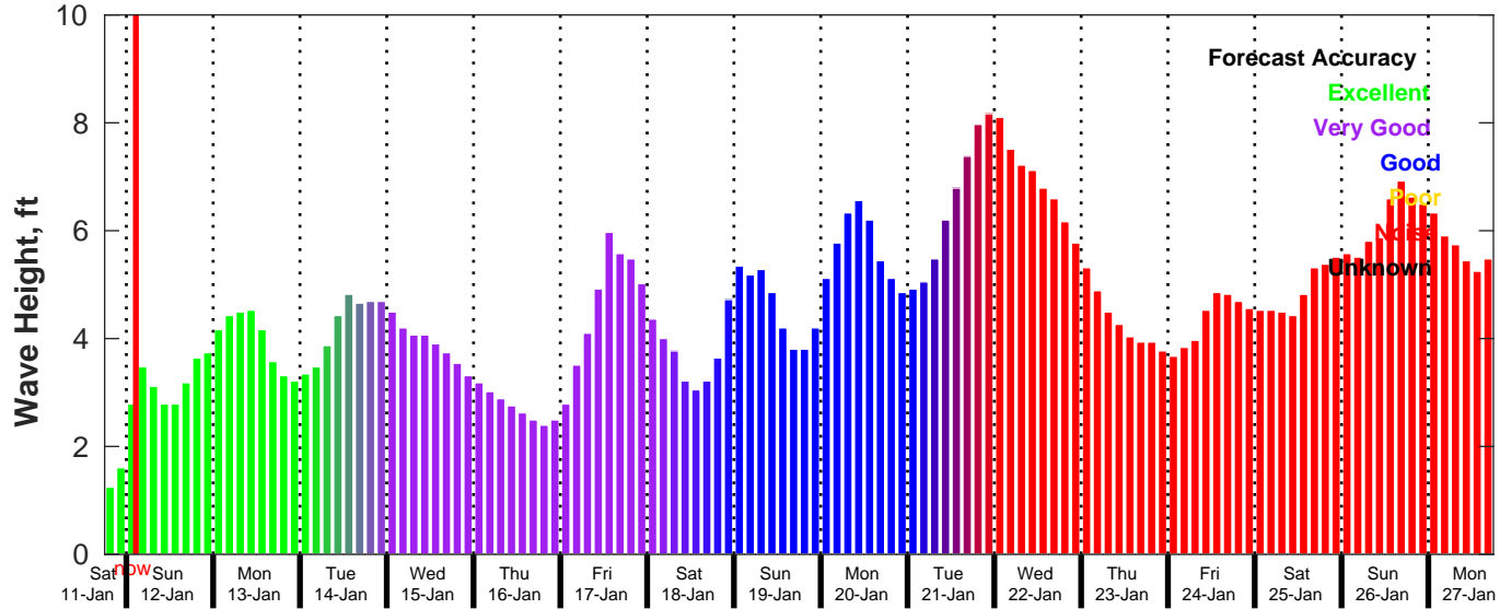
GFS Wave Forecast for NDBC 42092 from 11-Jan-2025 18:00:00 to 27-Jan-2025 18:00:00
