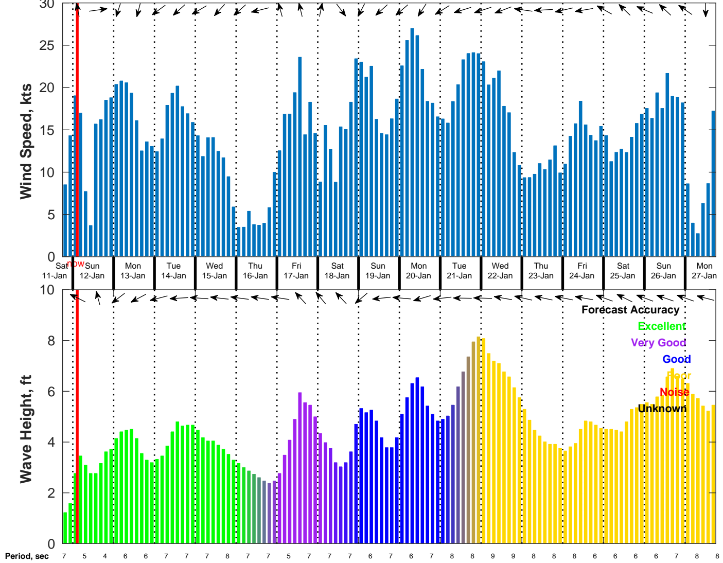
Wind & Wave Forecast for NDBC 42092 from 11-Jan-2025 18:00:00 to 27-Jan-2025 18:00:00
