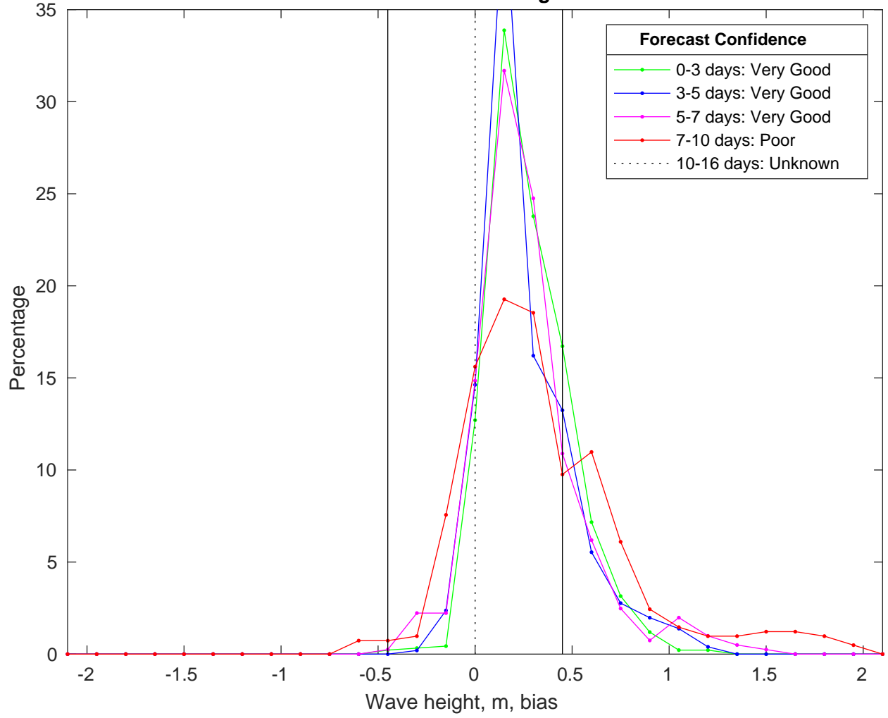
NDBC 44020 vs CMEMSWaves Bias Histogram: 12-Jan-2025
