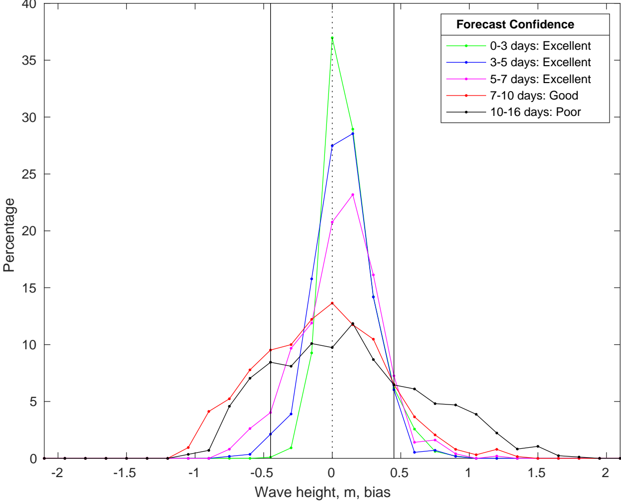
NDBC 44020 vs GFSWaves Bias Histogram: 12-Jan-2025
