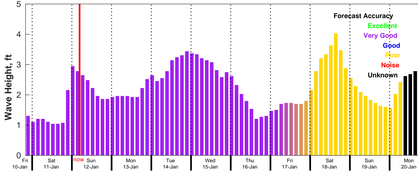
CMEMS Wave Forecast for NDBC 44020 from 10-Jan-2025 20:00:00 to 20-Jan-2025 20:00:00
