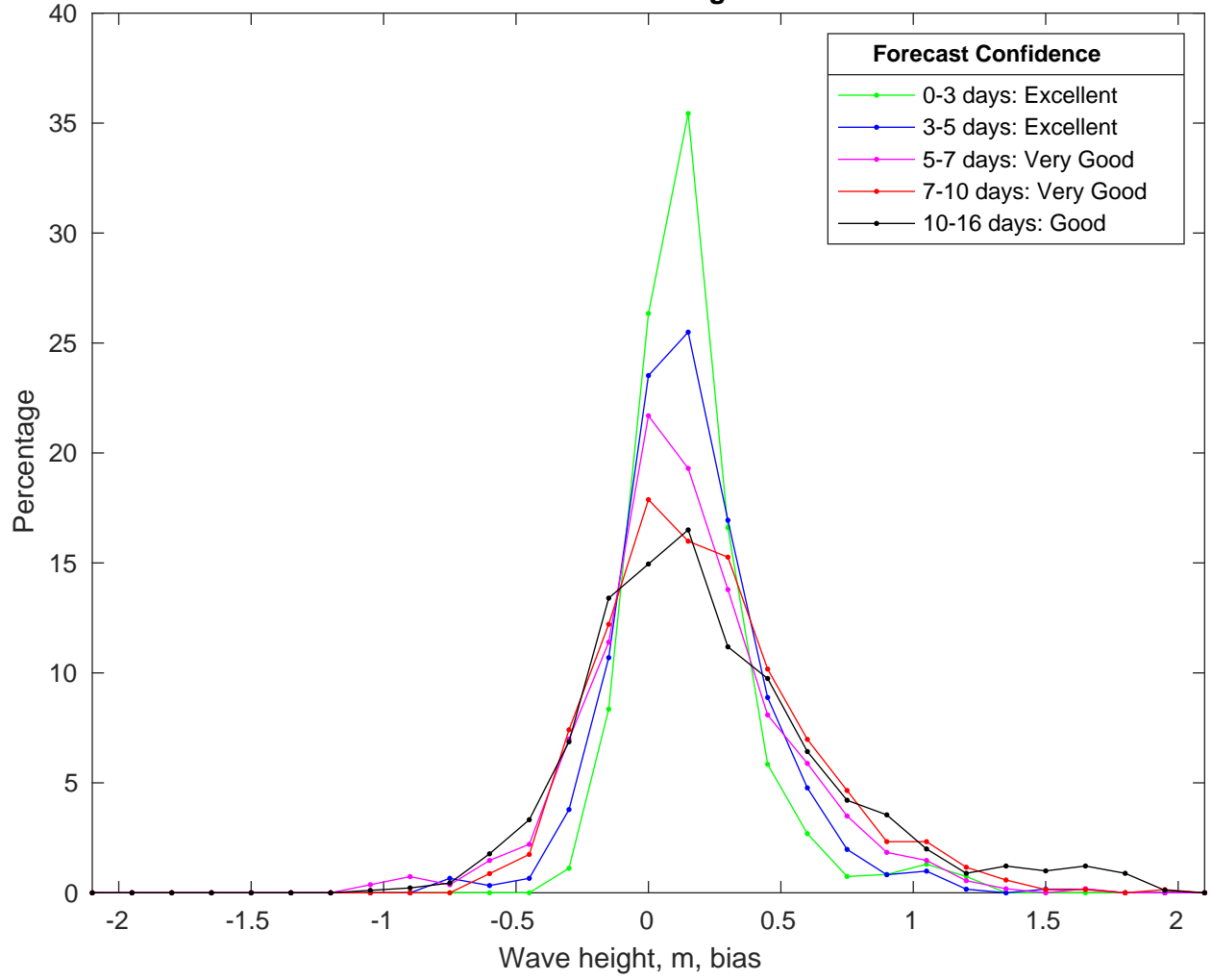
NDBC 44020 vs GFSWaves Bias Histogram: 26-Dec-2024
