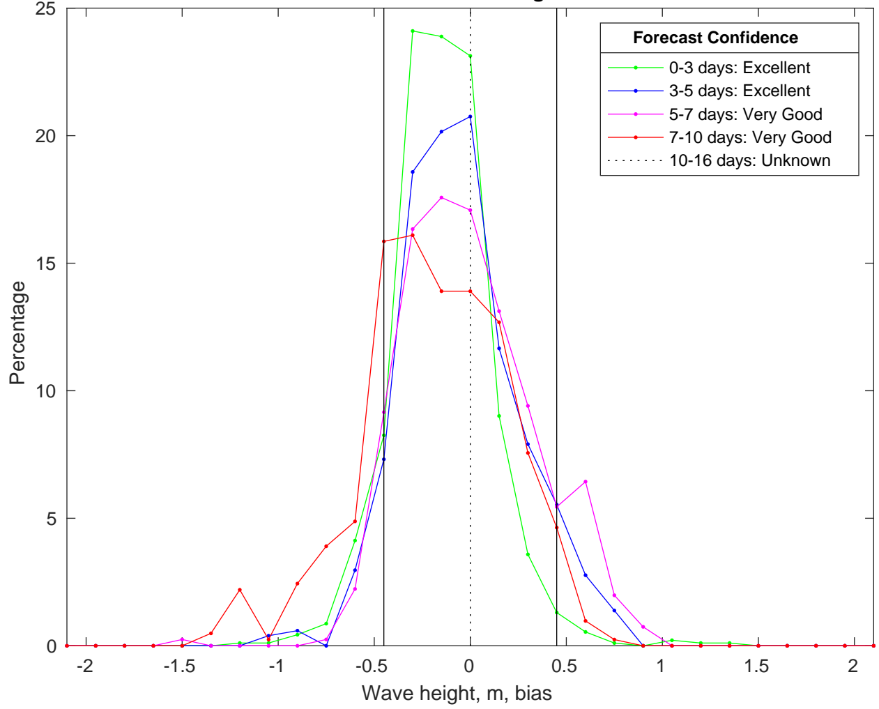
NDBC 46011 vs CMEMSWaves Bias Histogram: 12-Jan-2025
