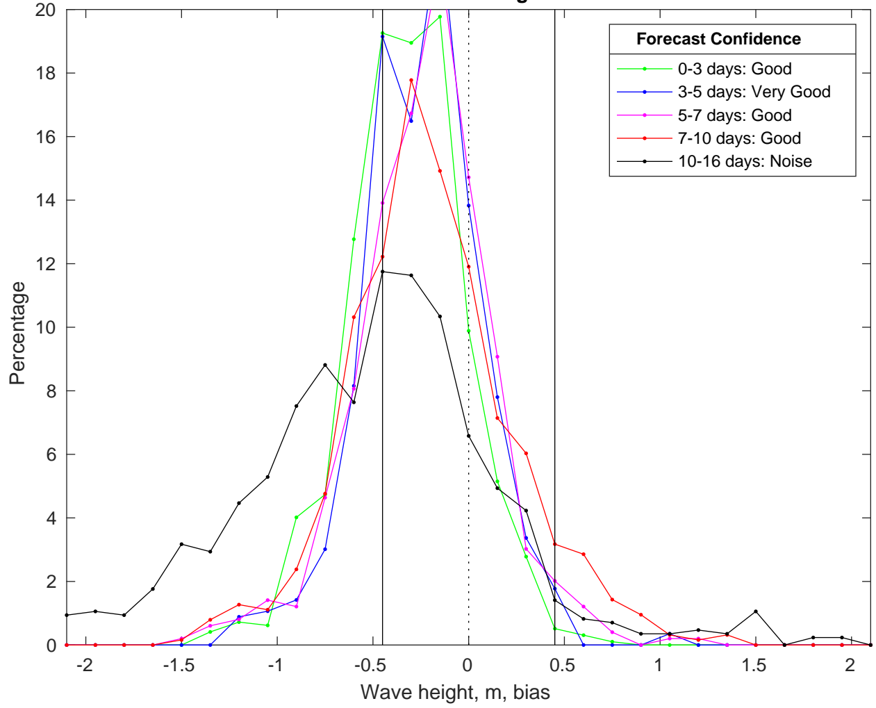
NDBC 46011 vs GFSWaves Bias Histogram: 12-Jan-2025
