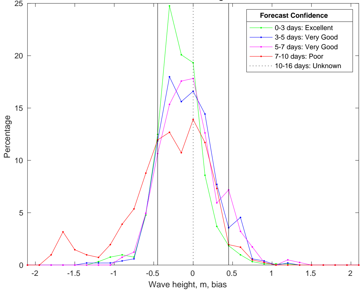
NDBC 46028 vs CMEMSWaves Bias Histogram: 12-Jan-2025
