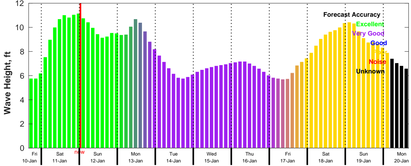
CMEMS Wave Forecast for NDBC 46028 from 10-Jan-2025 16:00:00 to 20-Jan-2025 16:00:00
