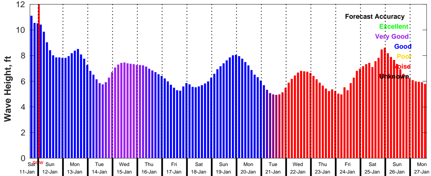
GFS Wave Forecast for NDBC 46028 from 11-Jan-2025 16:00:00 to 27-Jan-2025 16:00:00
