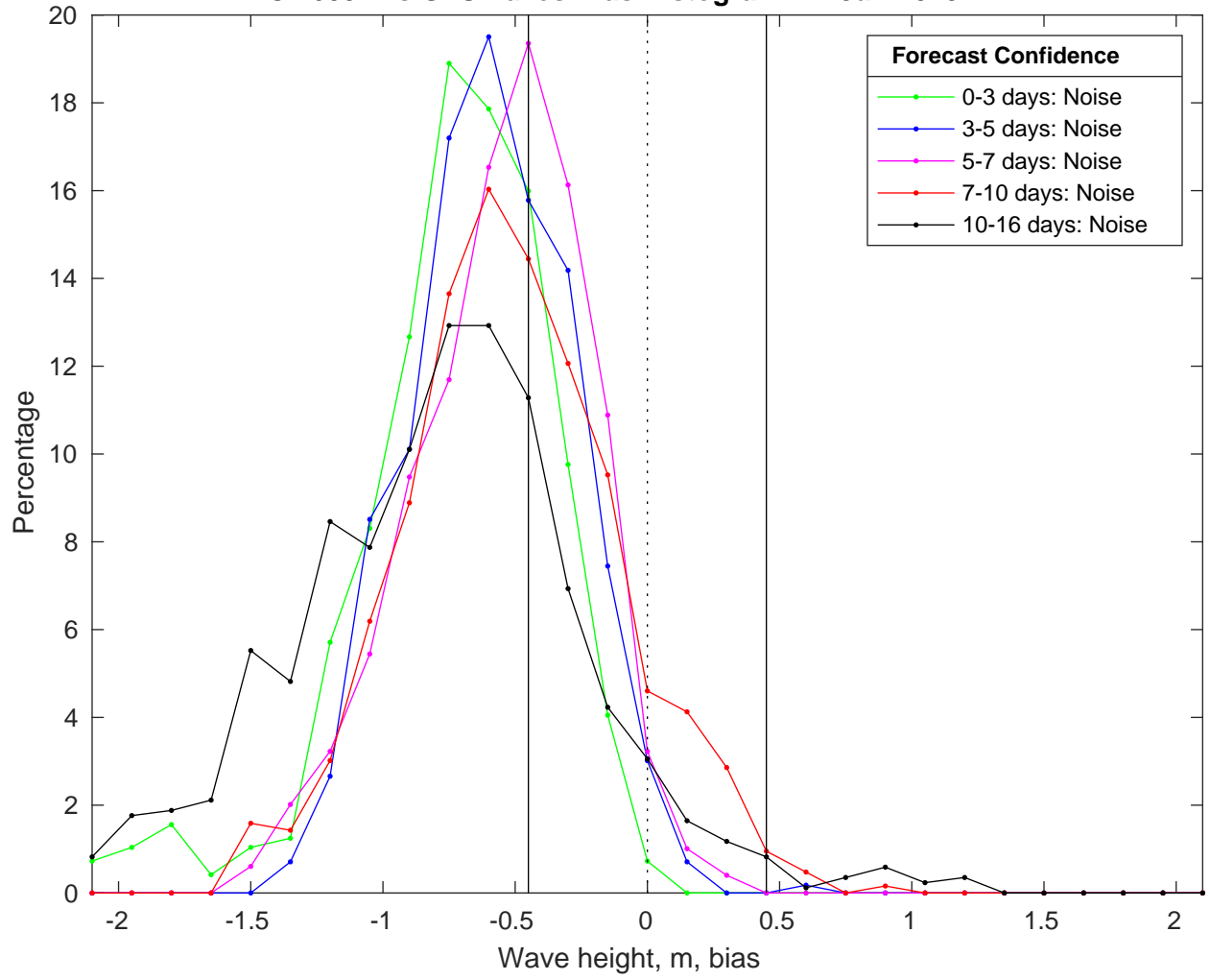
NDBC 46054 vs GFSWaves Bias Histogram: 12-Jan-2025
