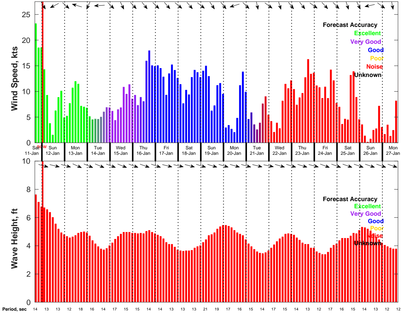
Wind & Wave Forecast for NDBC 46054 from 11-Jan-2025 16:00:00 to 27-Jan-2025 16:00:00
