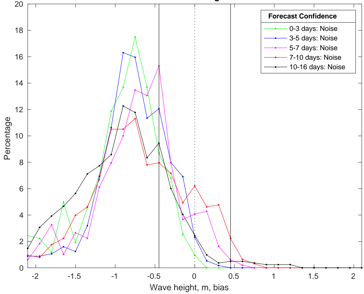
NDBC 46069 vs GFSWaves Bias Histogram: 12-Jan-2025
