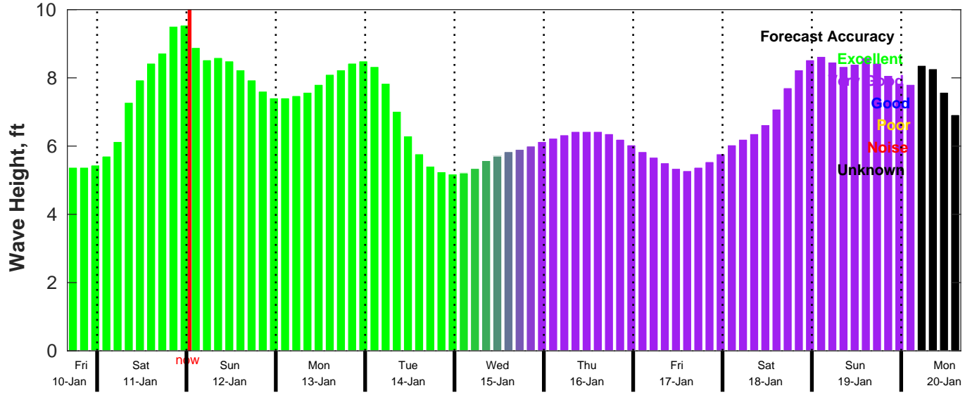
CMEMS Wave Forecast for NDBC 46069 from 10-Jan-2025 16:00:00 to 20-Jan-2025 16:00:00
