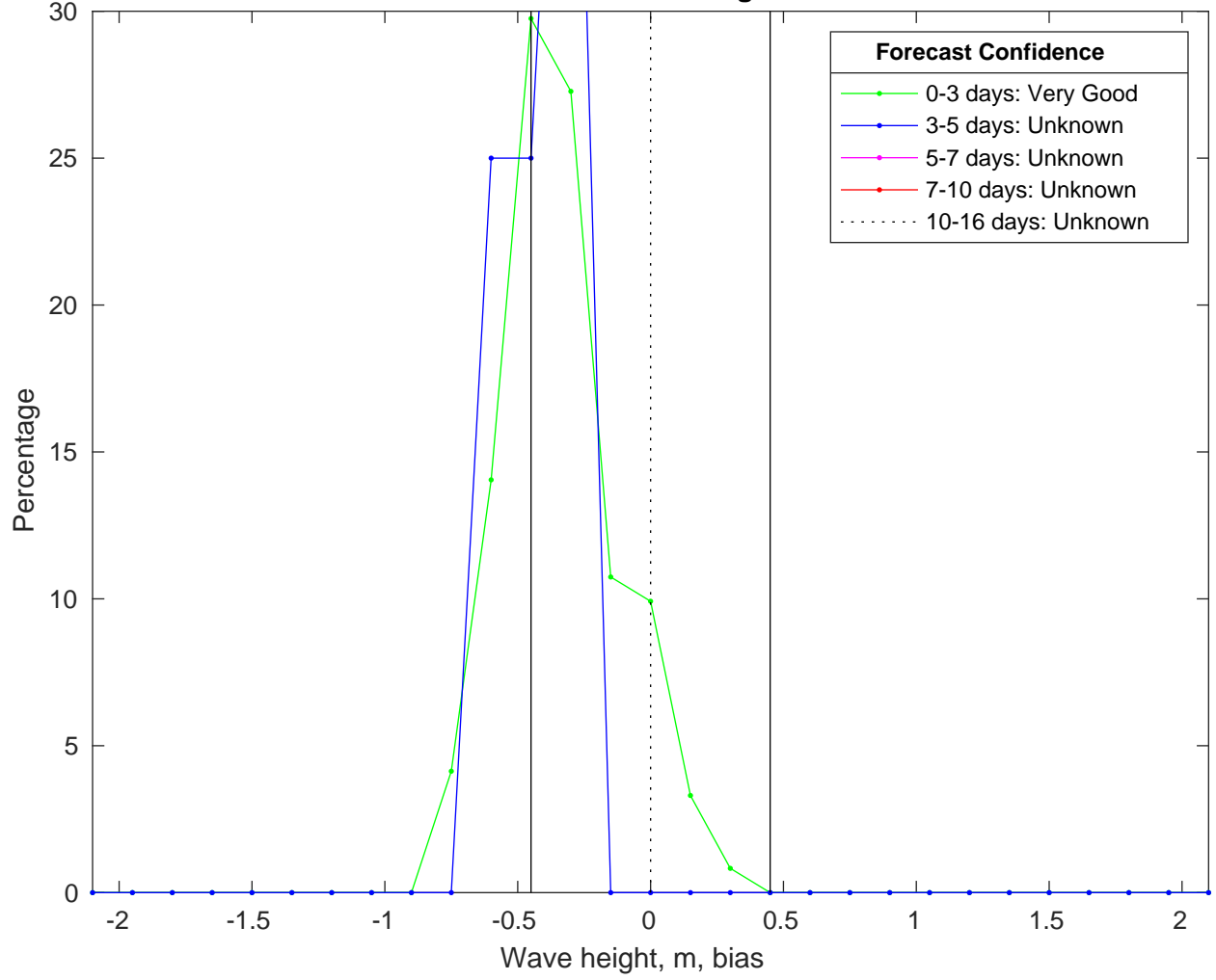
NDBC 51209 vs CMEMSWaves Bias Histogram: 12-Jan-2025
