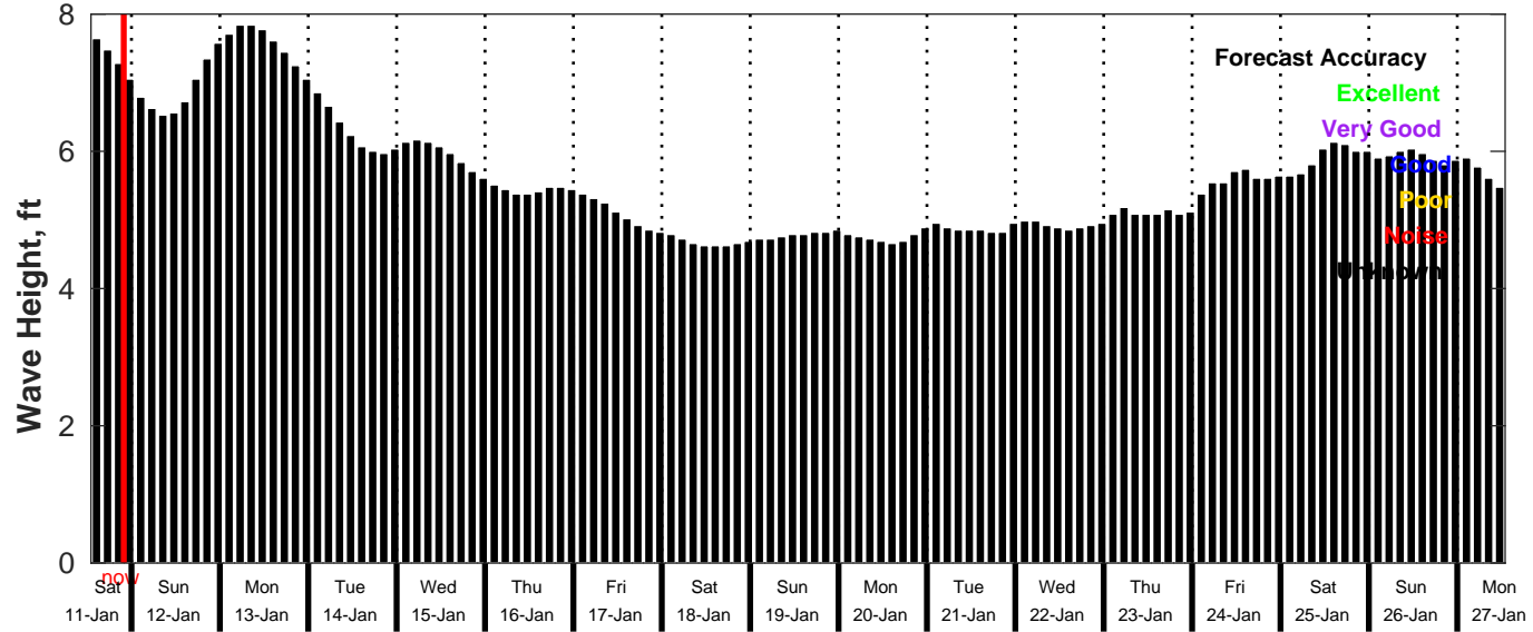
GFS Wave Forecast for NDBC 51209 from 11-Jan-2025 13:00:00 to 27-Jan-2025 13:00:00
