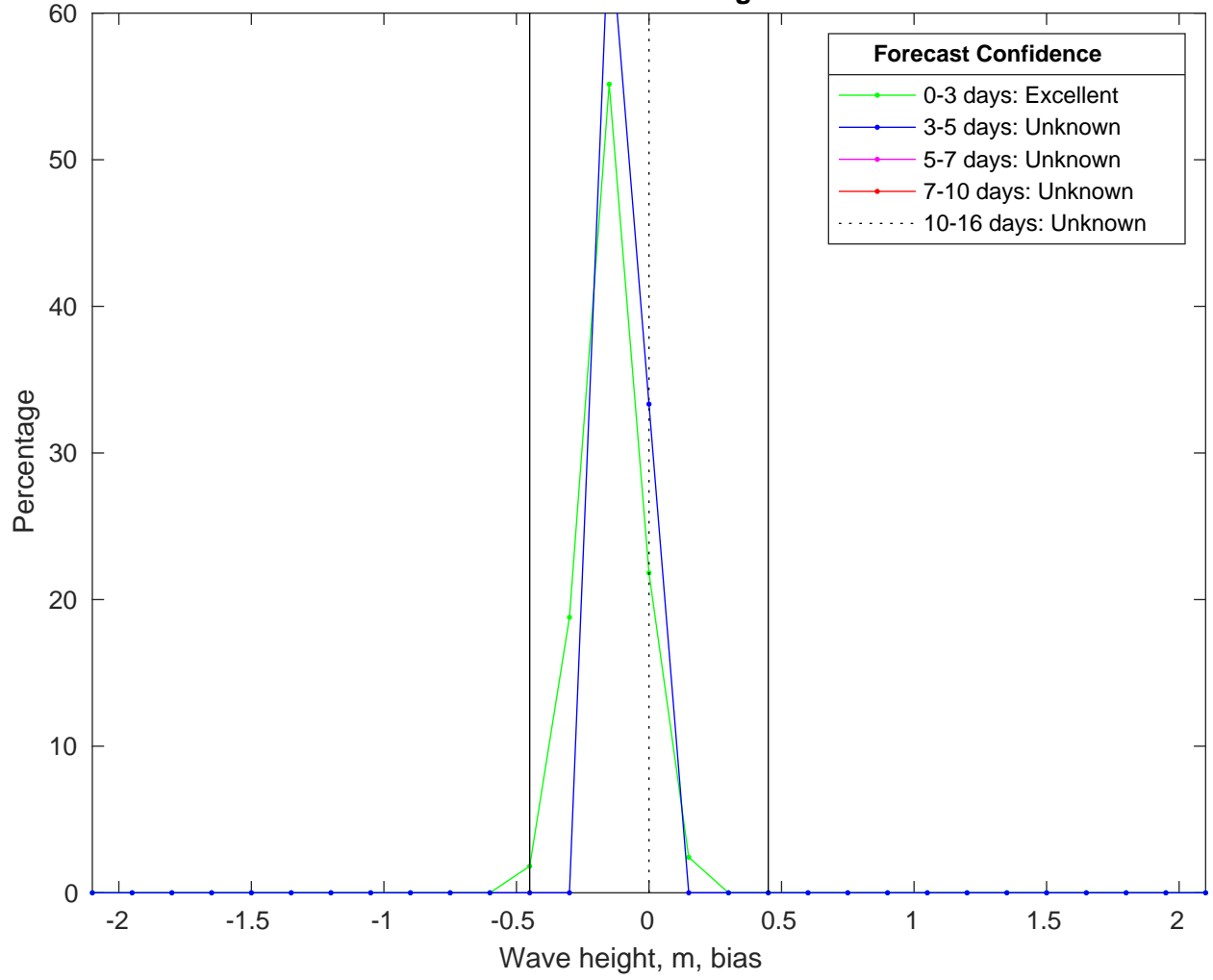
NDBC 52211 vs CMEMSWaves Bias Histogram: 12-Jan-2025
