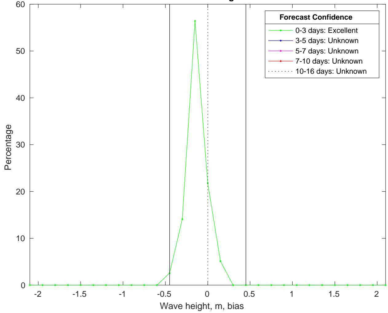
NDBC 52211 vs GFSWaves Bias Histogram: 12-Jan-2025
