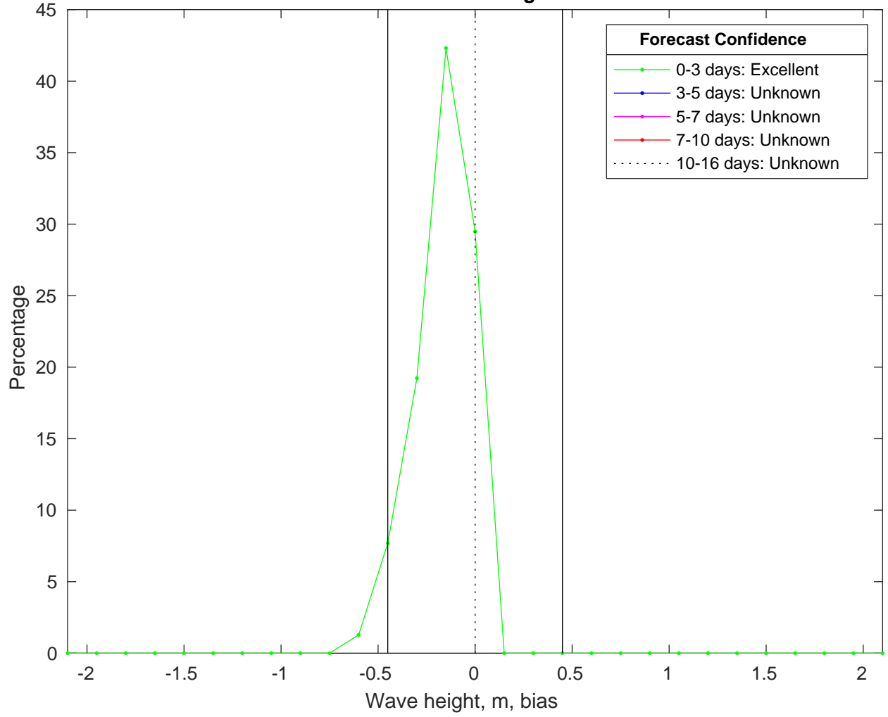
NDBC 52212 vs GFSWaves Bias Histogram: 12-Jan-2025
