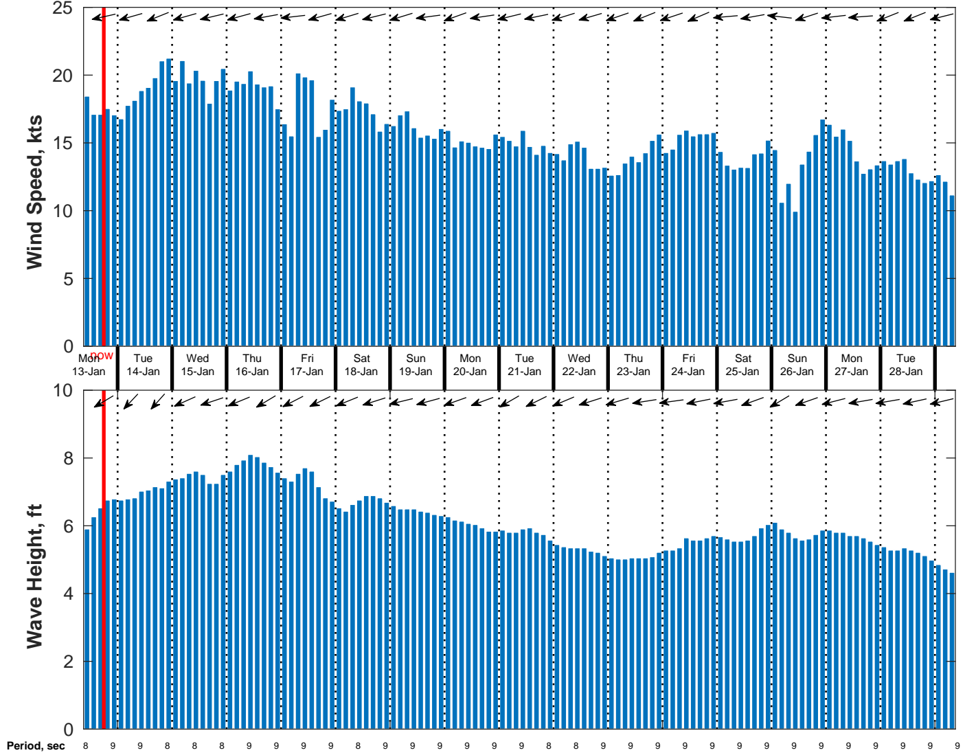
Wind & Wave Forecast for NDBC 52212 from 12-Jan-2025 09:00:00 to 28-Jan-2025 09:00:00
