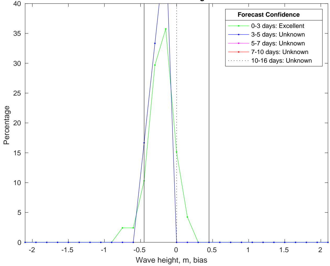
NDBC 52213 vs CMEMSWaves Bias Histogram: 12-Jan-2025
