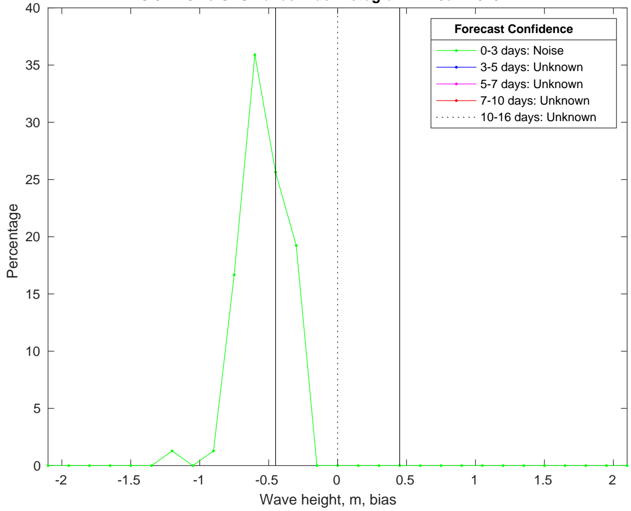
NDBC 52213 vs GFSWaves Bias Histogram: 12-Jan-2025
