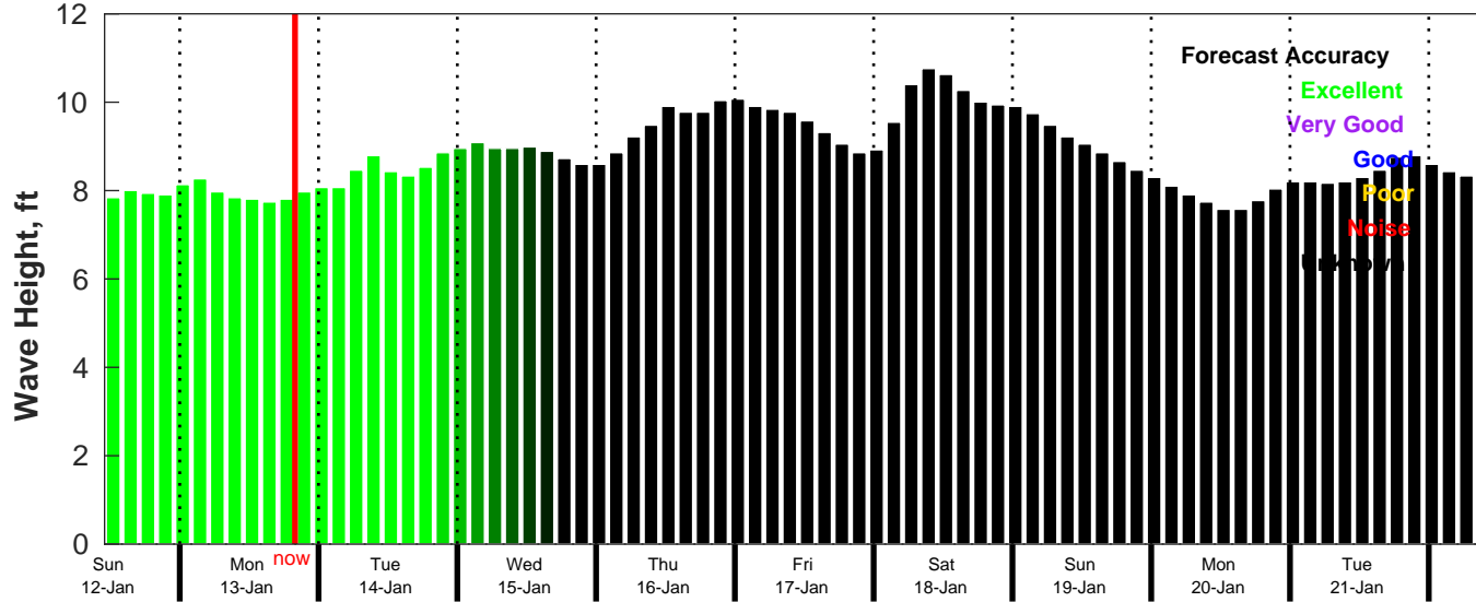
CMEMS Wave Forecast for NDBC 52213 from 11-Jan-2025 11:00:00 to 21-Jan-2025 11:00:00
