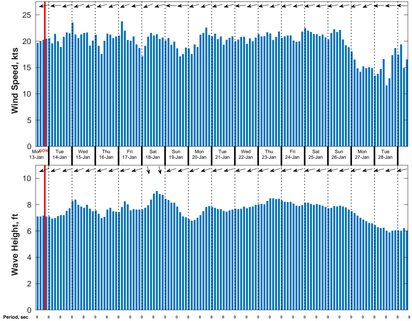
Wind & Wave Forecast for NDBC 52213 from 12-Jan-2025 11:00:00 to 28-Jan-2025 11:00:00
