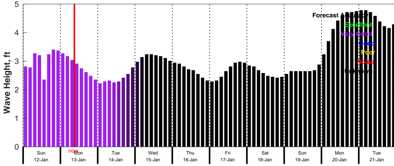
CMEMS Wave Forecast for NDBC 62305 from 11-Jan-2025 00:00:00 to 21-Jan-2025 00:00:00
