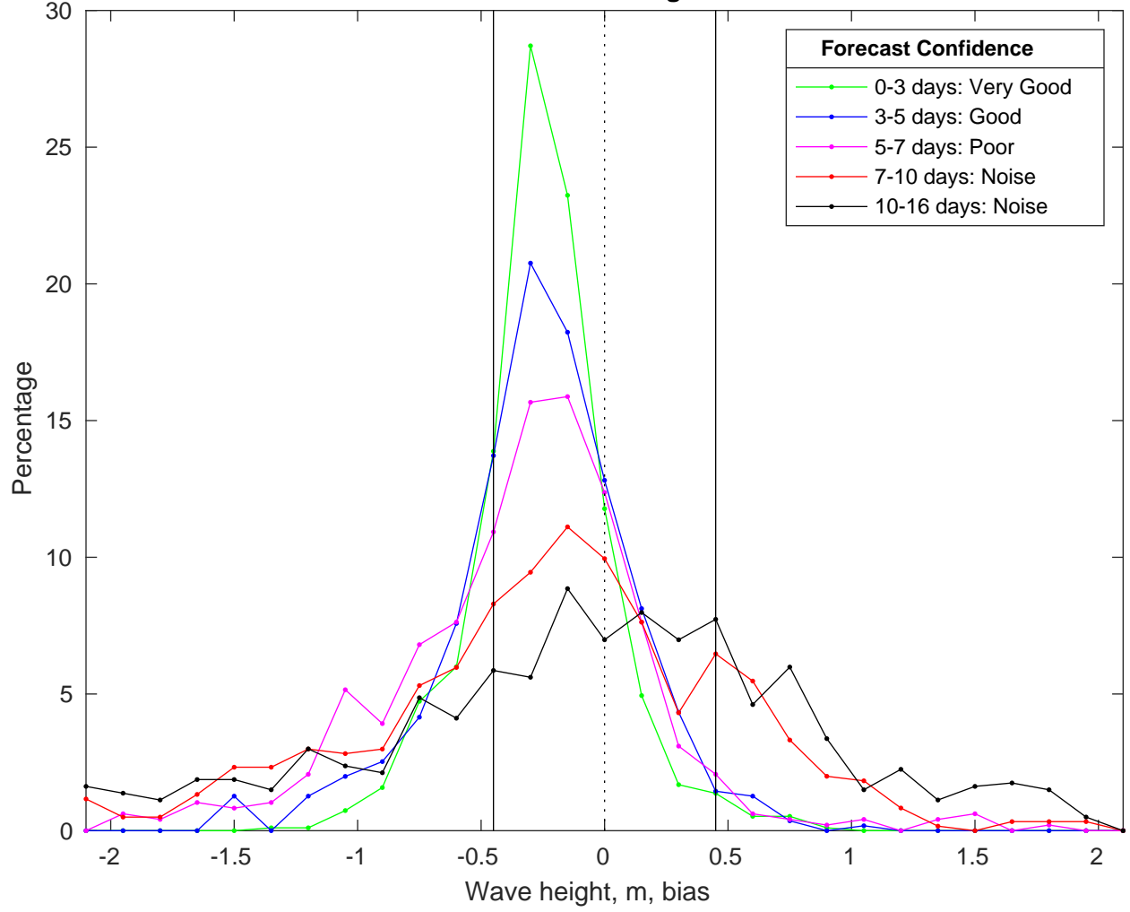
NDBC 41004 vs GFSWaves Bias Histogram: 13-Jan-2025
