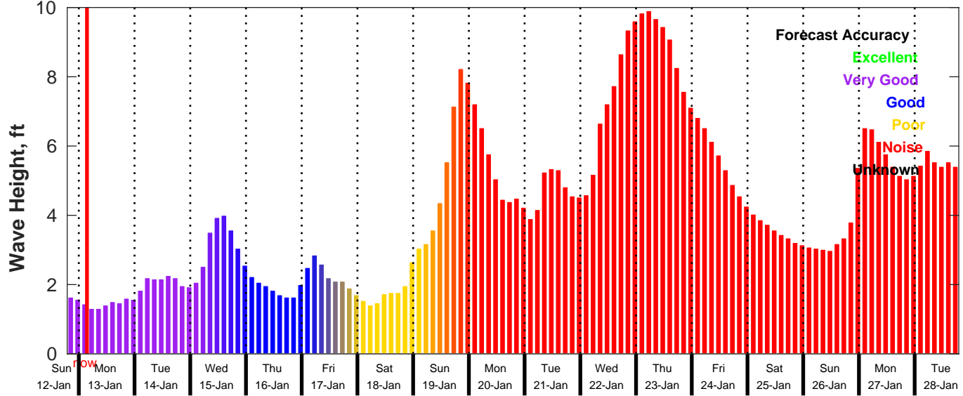
GFS Wave Forecast for NDBC 41004 from 12-Jan-2025 19:00:00 to 28-Jan-2025 19:00:00
