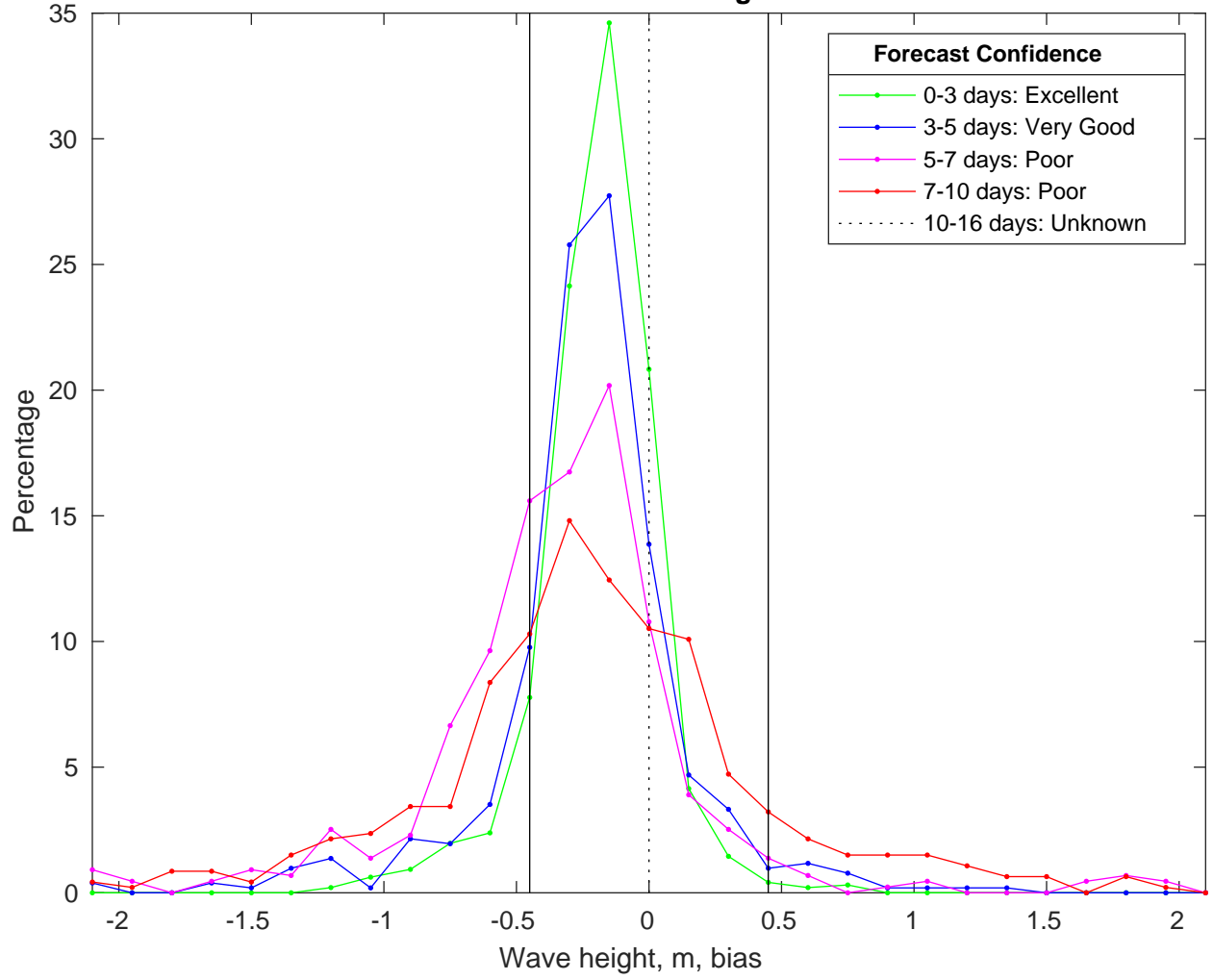
NDBC 41013 vs CMEMSWaves Bias Histogram: 13-Jan-2025
