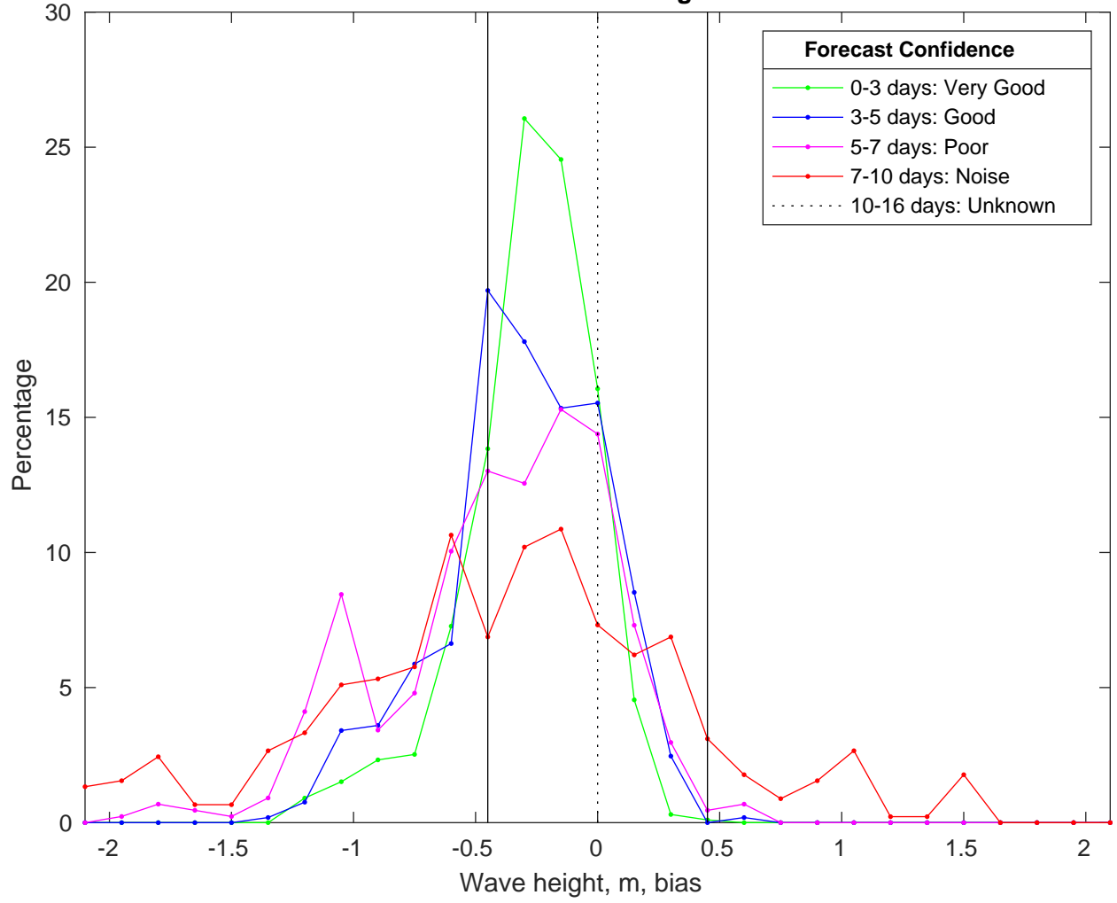
NDBC 42019 vs CMEMSWaves Bias Histogram: 13-Jan-2025
