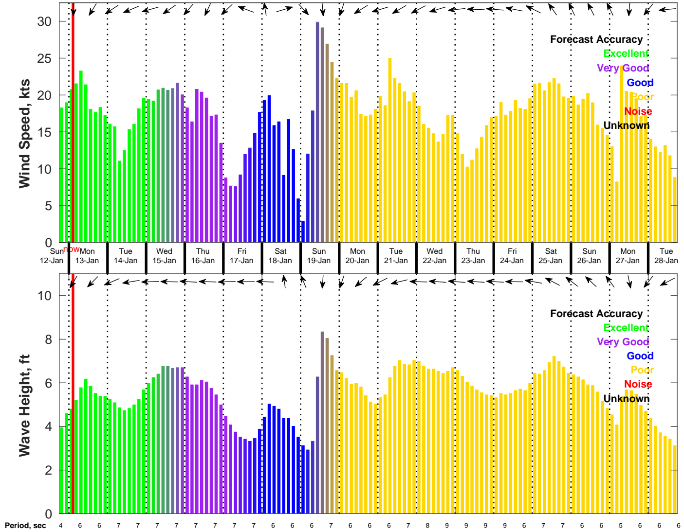
Wind & Wave Forecast for NDBC 42019 from 12-Jan-2025 18:00:00 to 28-Jan-2025 18:00:00
