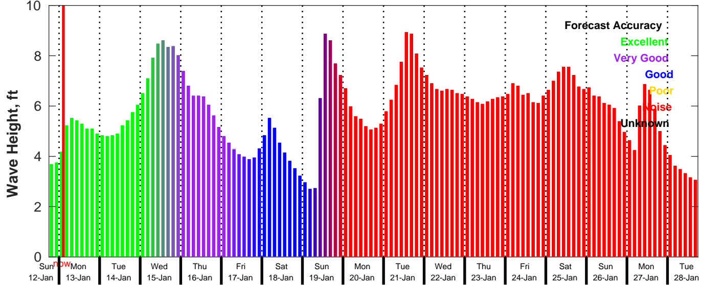
GFS Wave Forecast for NDBC 42020 from 12-Jan-2025 18:00:00 to 28-Jan-2025 18:00:00
