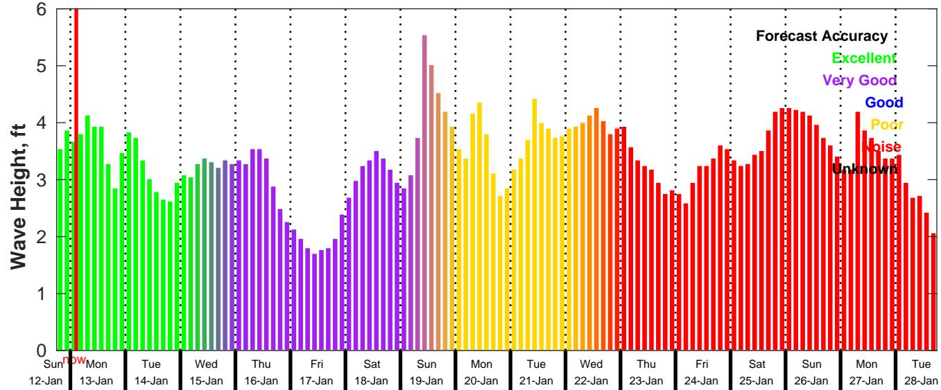
GFS Wave Forecast for NDBC 42035 from 12-Jan-2025 18:00:00 to 28-Jan-2025 18:00:00
