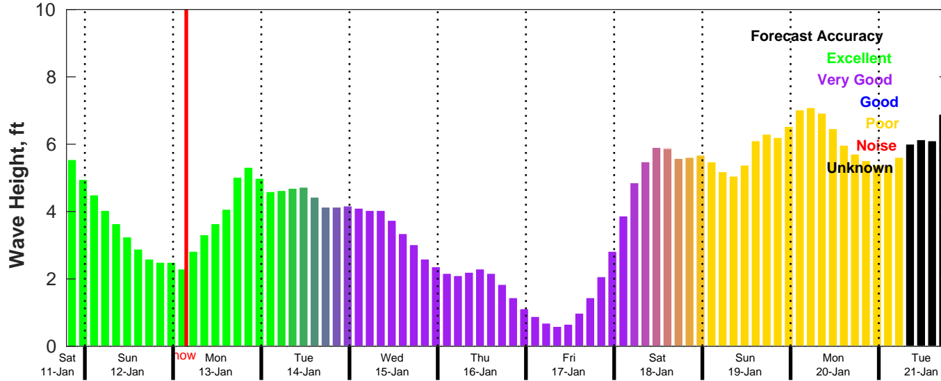
CMEMS Wave Forecast for NDBC 42036 from 11-Jan-2025 19:00:00 to 21-Jan-2025 19:00:00
