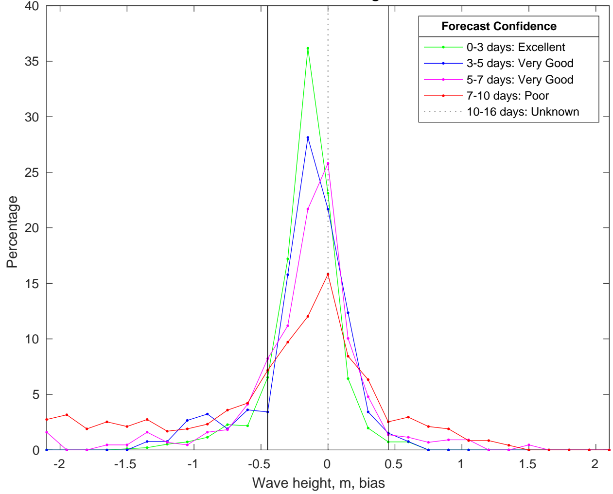
NDBC 42040 vs CMEMSWaves Bias Histogram: 13-Jan-2025
