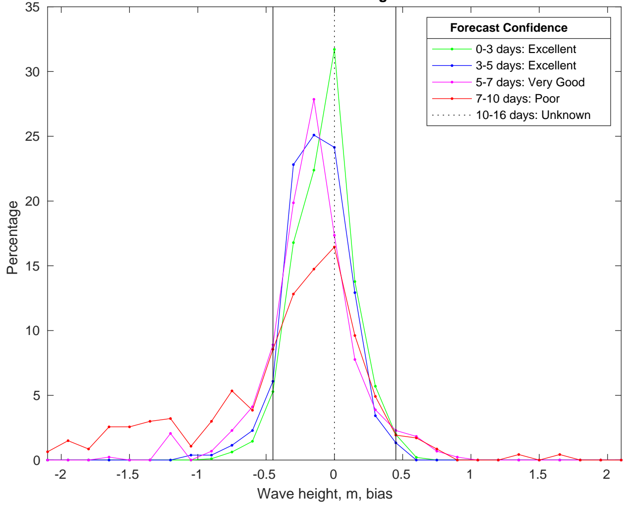
NDBC 42084 vs CMEMSWaves Bias Histogram: 13-Jan-2025
