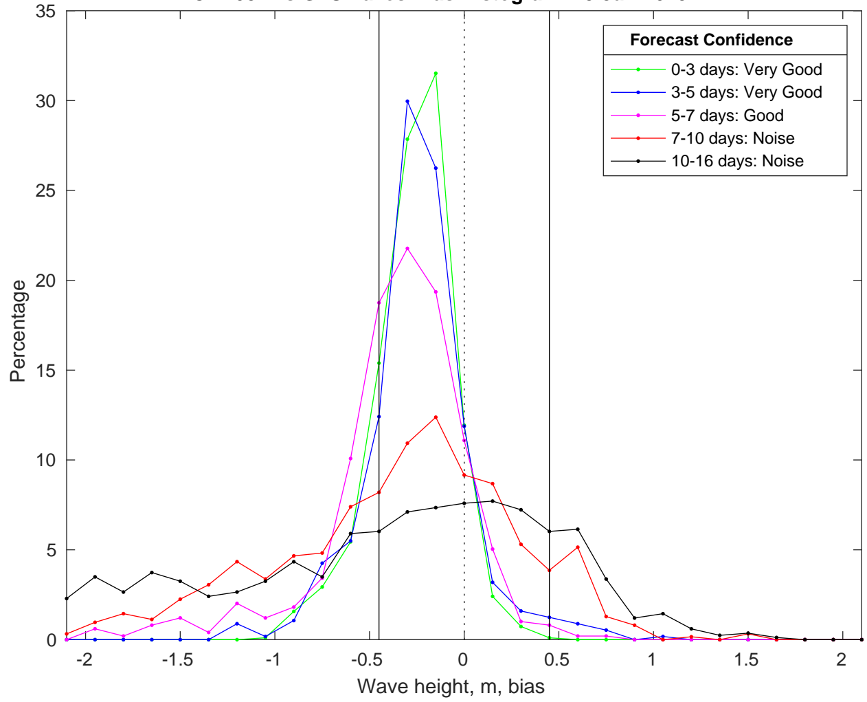
NDBC 42084 vs GFSWaves Bias Histogram: 13-Jan-2025
