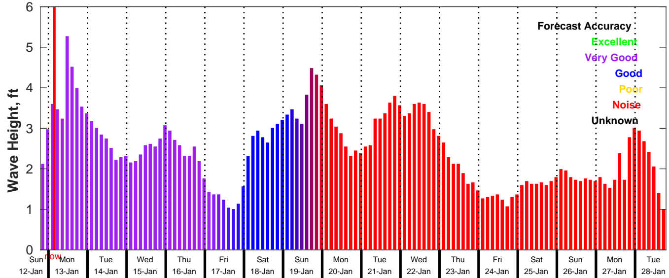
GFS Wave Forecast for NDBC 42084 from 12-Jan-2025 19:00:00 to 28-Jan-2025 19:00:00
