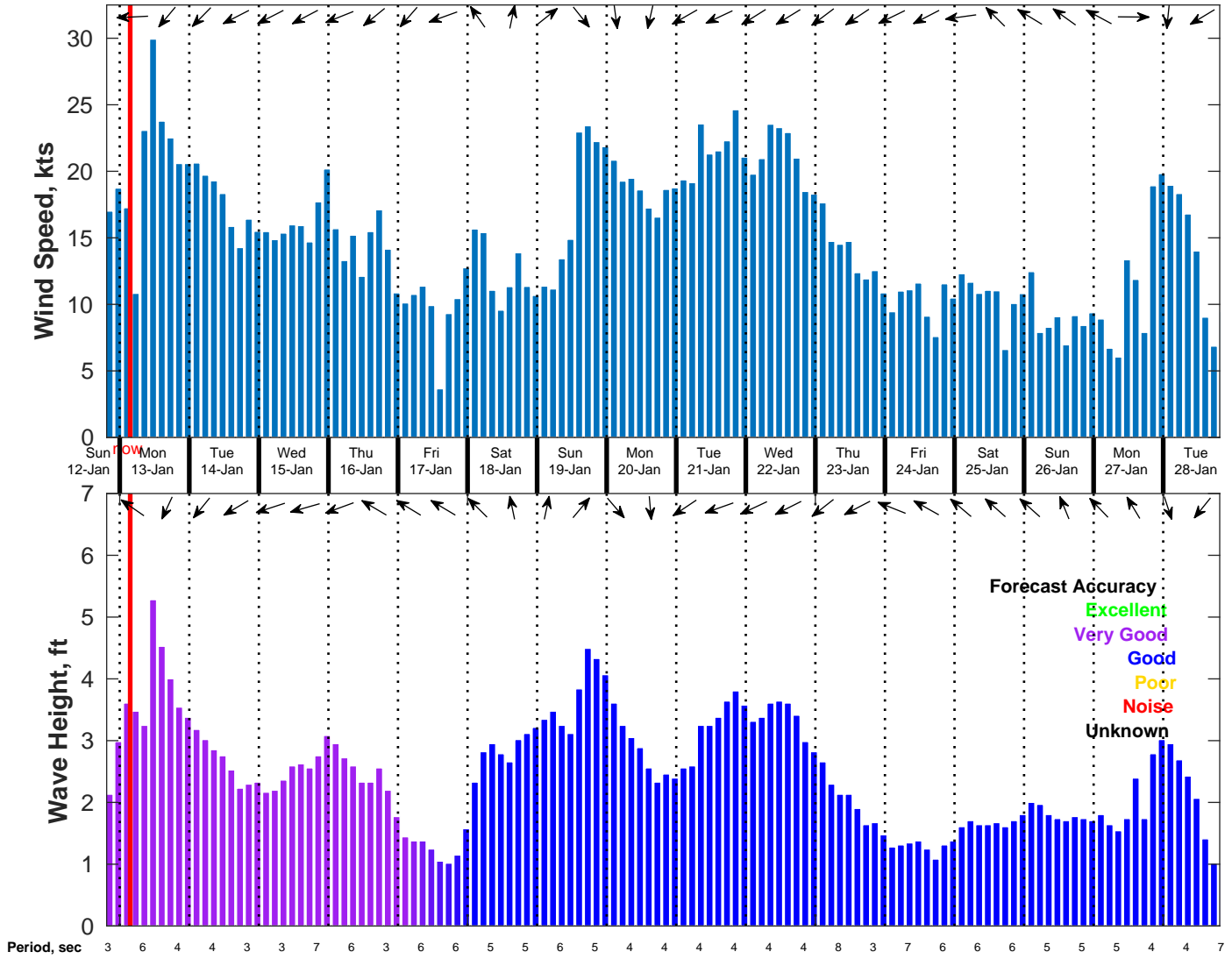
Wind & Wave Forecast for NDBC 42084 from 12-Jan-2025 19:00:00 to 28-Jan-2025 19:00:00
