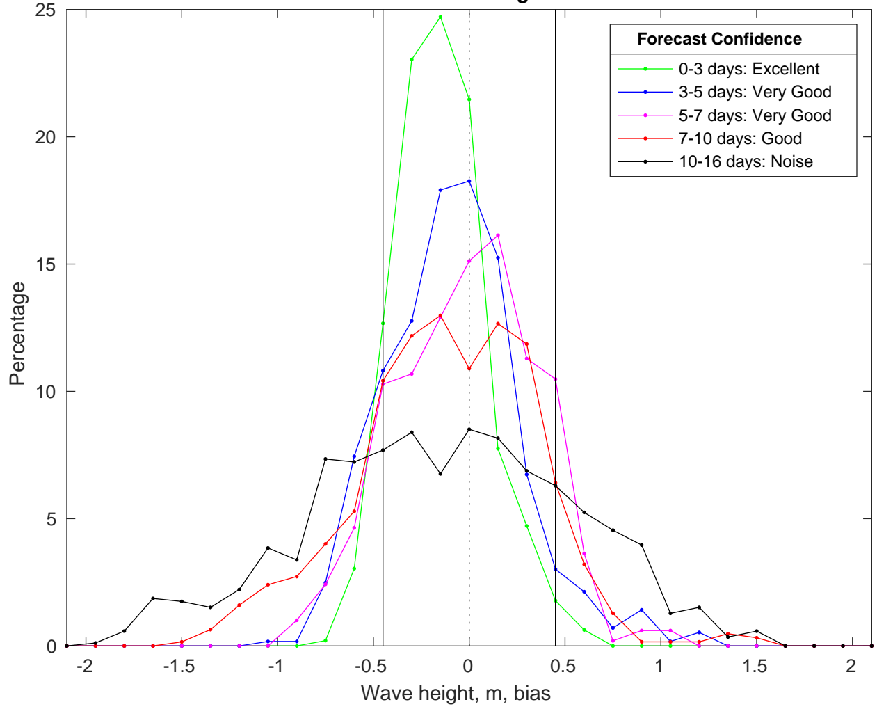
NDBC 42092 vs GFSWaves Bias Histogram: 13-Jan-2025
