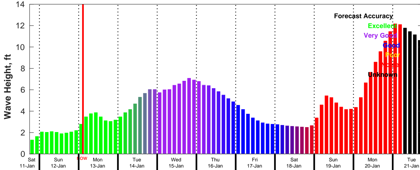
CMEMS Wave Forecast for NDBC 42092 from 11-Jan-2025 18:00:00 to 21-Jan-2025 18:00:00
