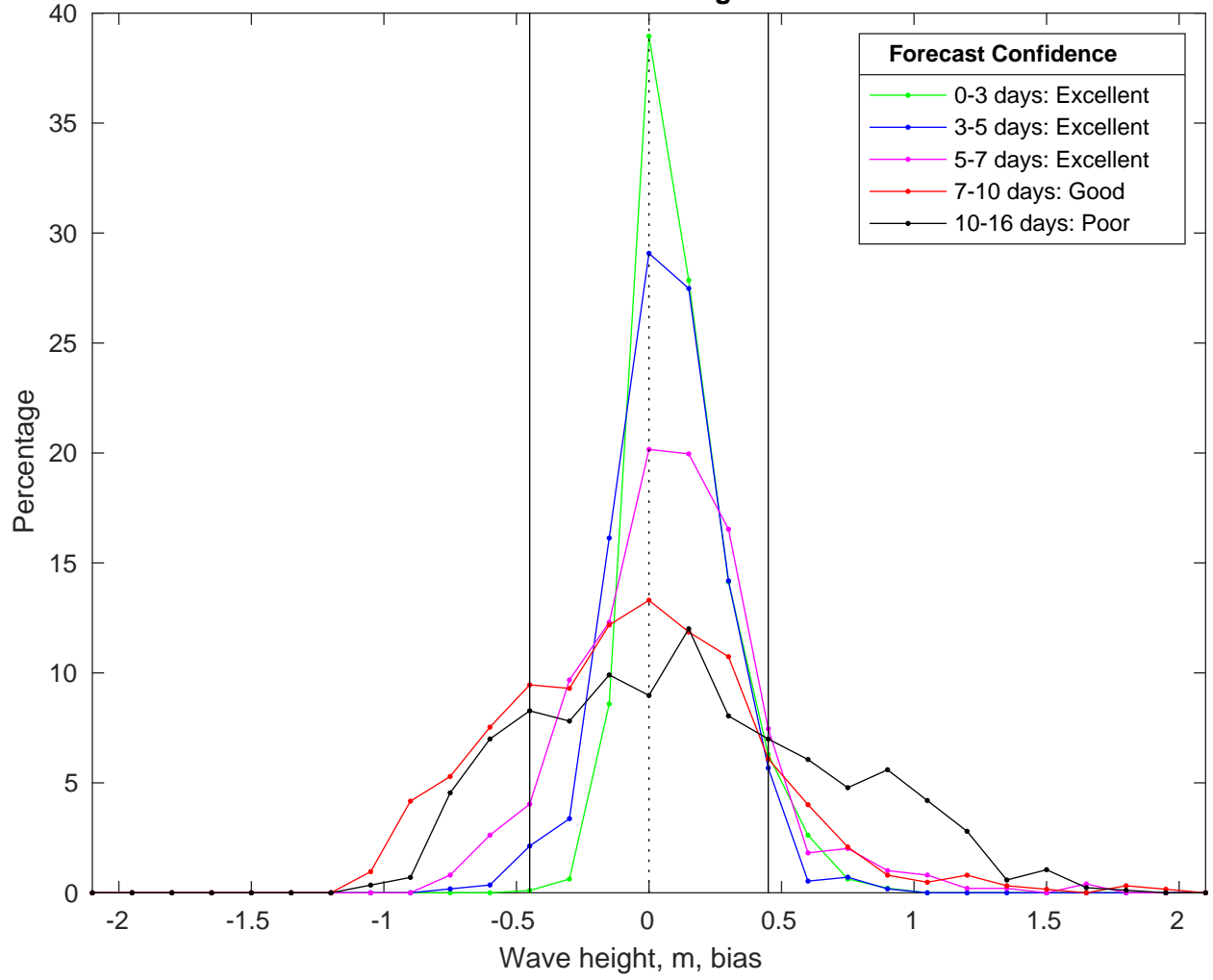
NDBC 44020 vs GFSWaves Bias Histogram: 13-Jan-2025
